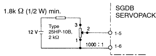
Type 25HP-10B
