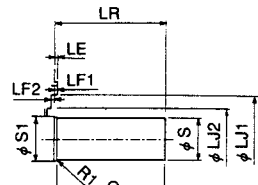
Detailed View of Shaft End for SGMG-55A2AAB and -75A2AAB
