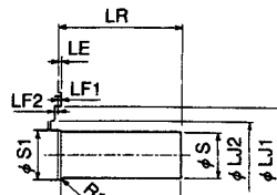
Detailed View of Shaft End
