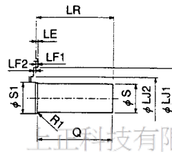
Detailed View of Shaft End for SGMG-1AASAAB and -1EASAAB
