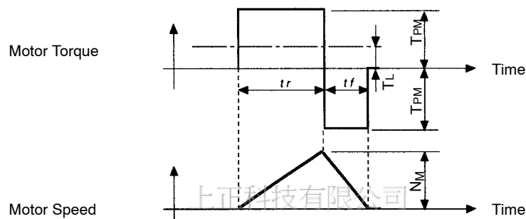
Motor Torque (size) - Motor Speed Timing Chart
