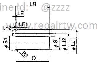
Detailed View of Shaft End for SGMG-20A2A to -75A2A
