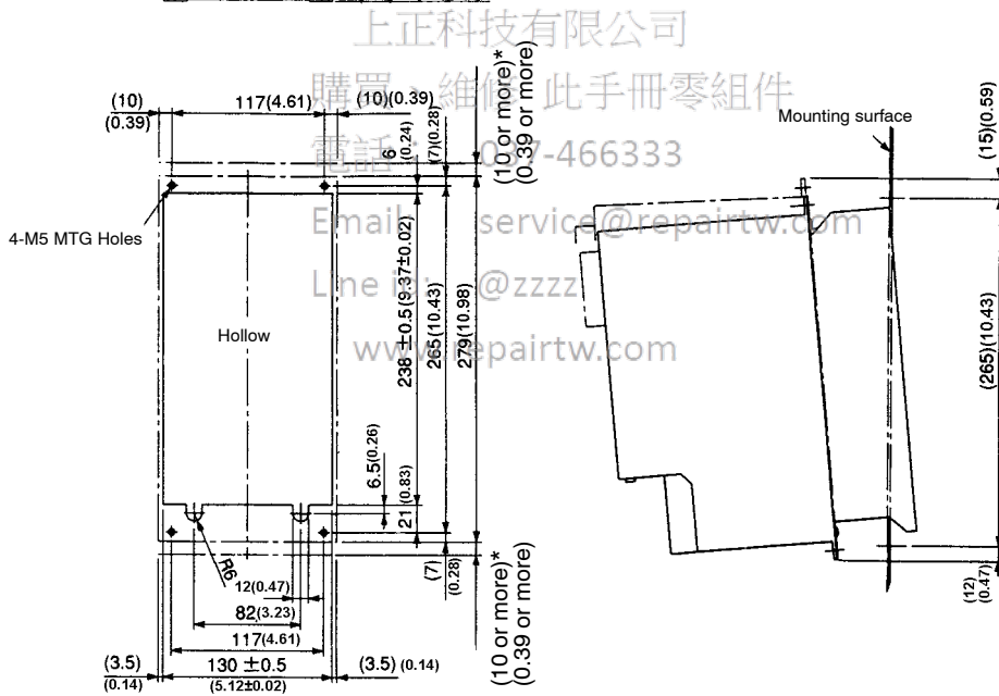
Mounting Surface Diagram
