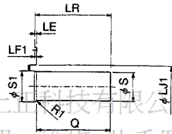
Detailed View of Shaft End for SGMG-20A2A to -75A2A
