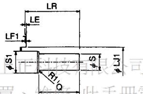
Detailed View of Shaft End for SGMG-12ASBAB to -30ASBAB Email: service@repairtw.com
