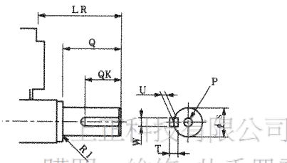
B : Straight with Key and Shaft End Tap
