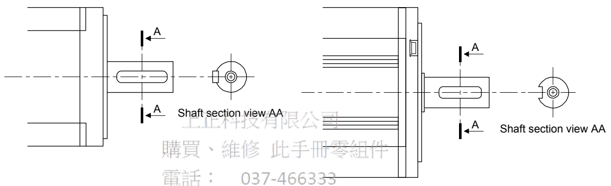
Key shaft (with 2 round end key)
