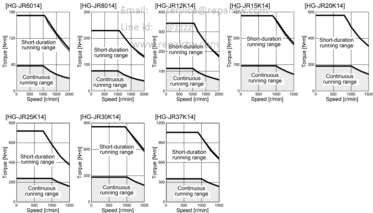
(c) 1000 r/min series
