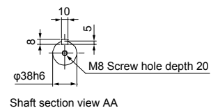
Shaft section view AA
