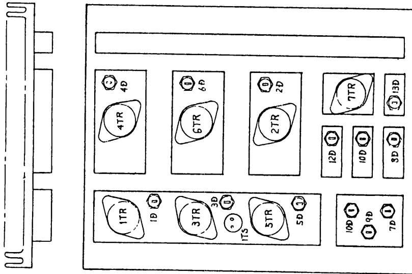
PARTS LAYOUT OF HEAT SINK (View Arrow A)
